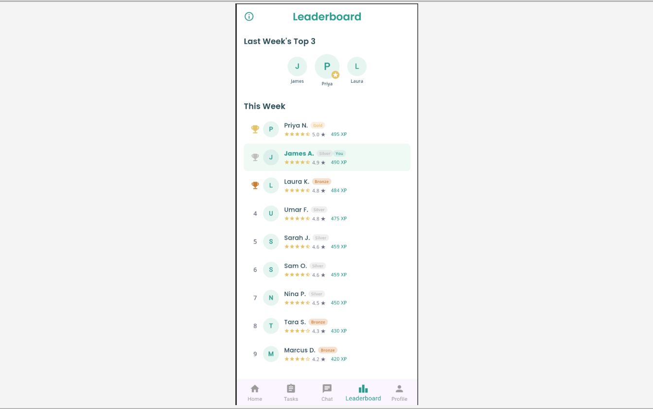
Leaderboard screen
