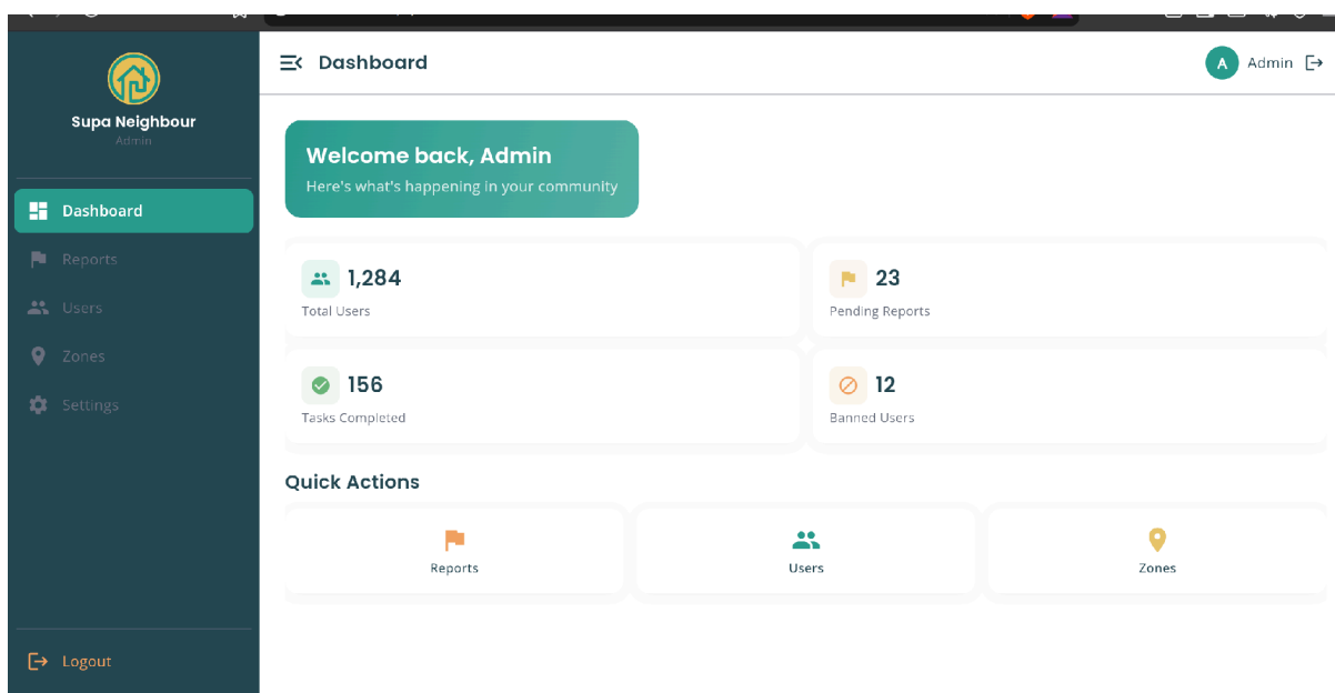
Dashboard overview
