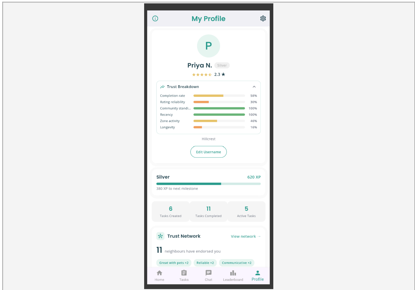
Profile screen
