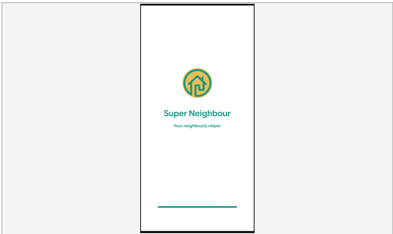
Splash screen
