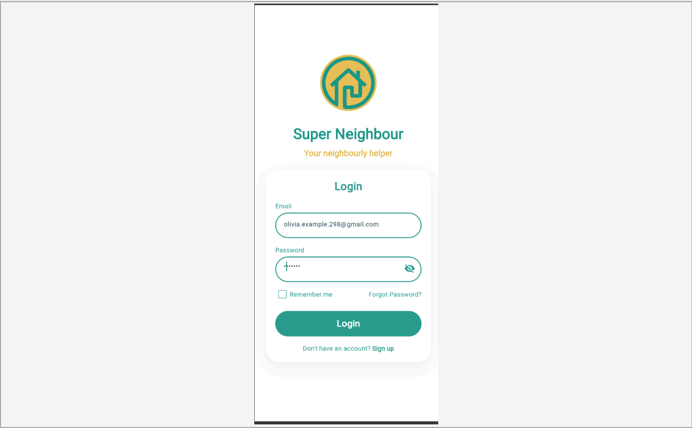
Login screen
