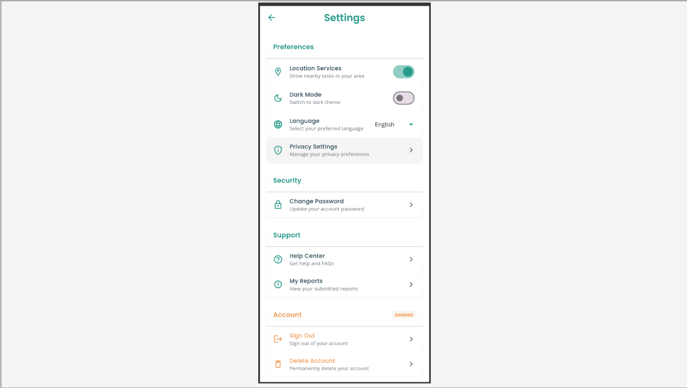
Settings screen
