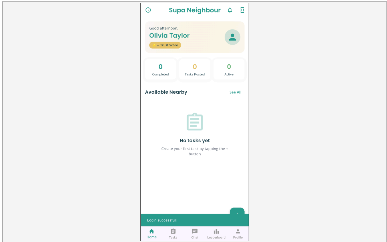
Home screen
